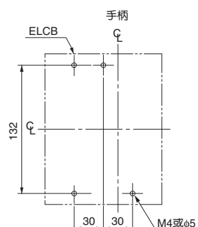
带外部操作手柄(V, N)
