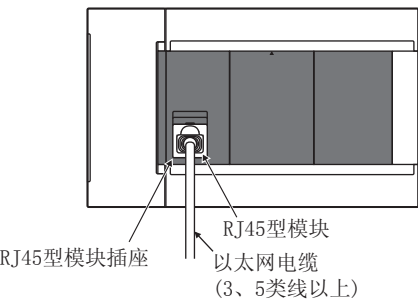
[CPU模块]
