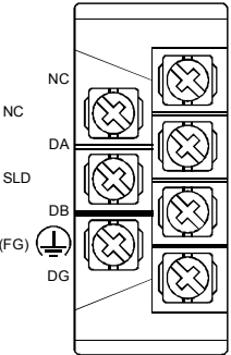
[盖子打开以后的端子排图]
